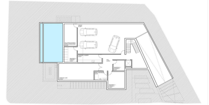
PLANTA SOTANO / BASEMENT FLOOR
