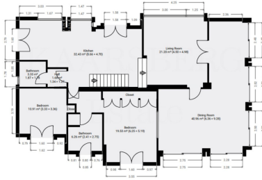
OTTO SCALE ground floor
